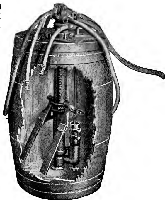
Pomona Spray Pump
